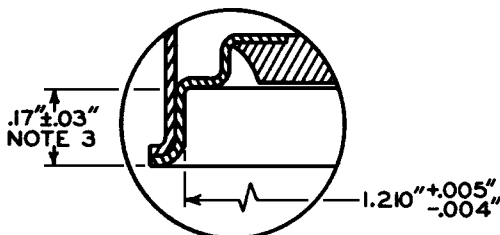
DETAIL B
